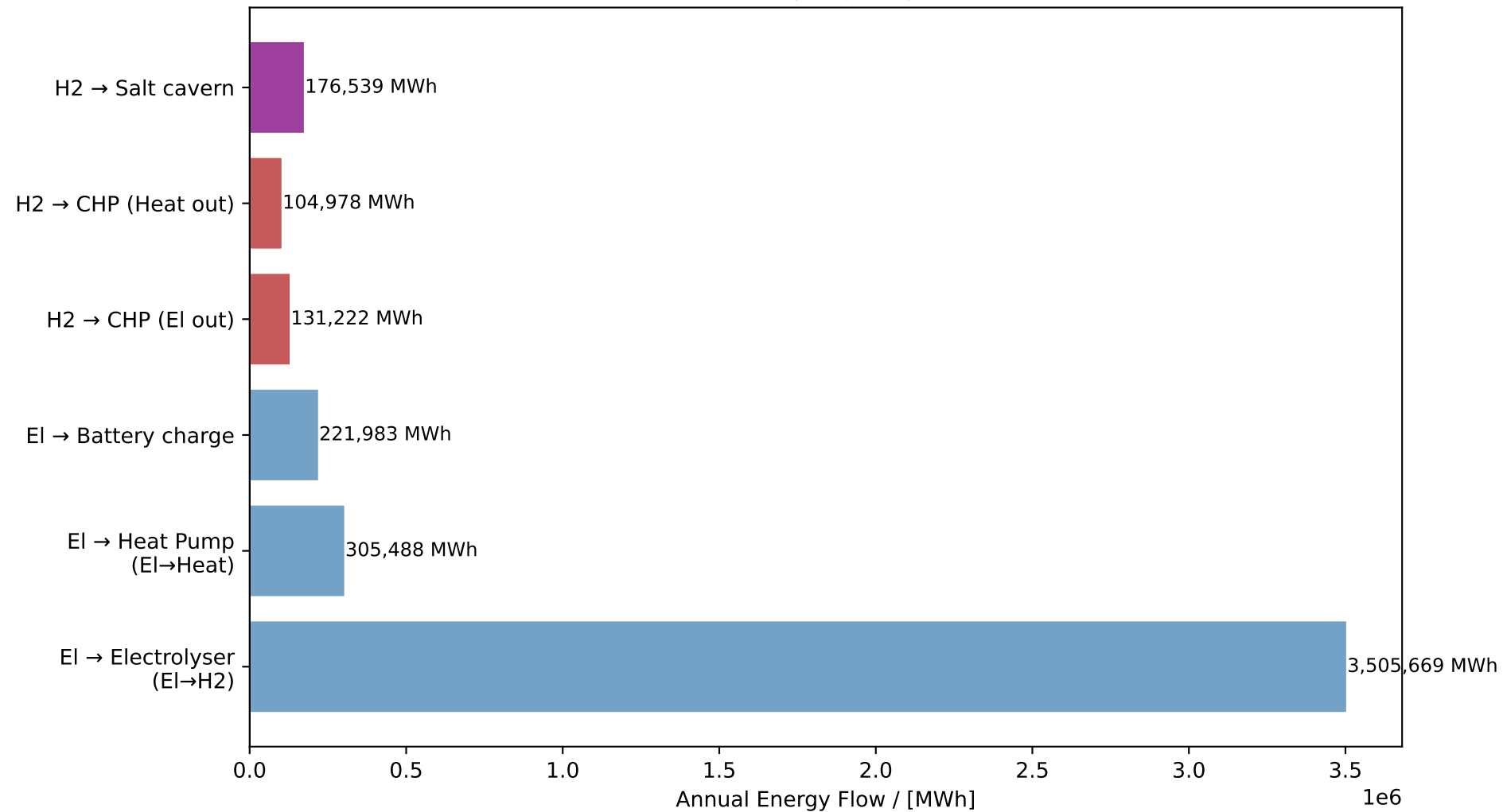
Annual Cross-Sector Energy Flows (Sector Coupling Magnitude)
